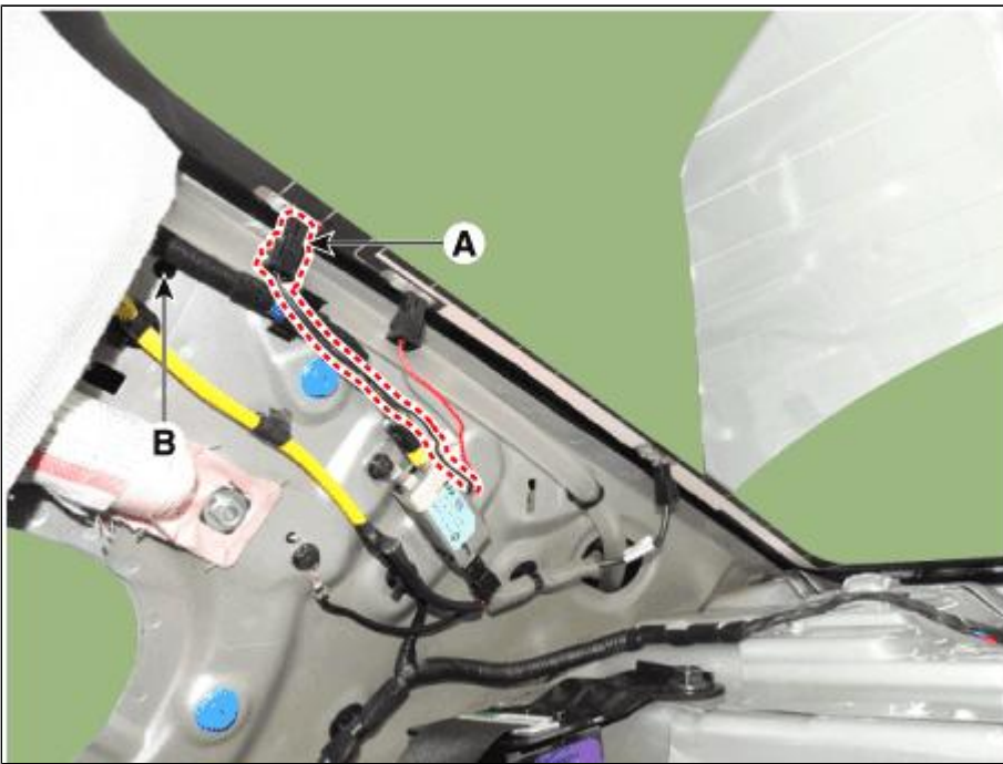
(2) FM1/FM2 antenna (RH side rear pillar)
